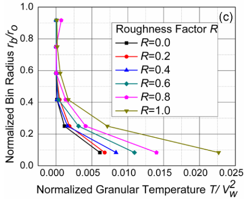
(Color online) Figure 6(c): Normalized granular temperature vs. radial location as a function of the roughness factor R .
