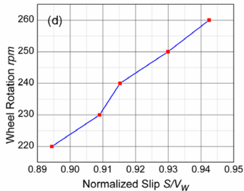
(Color online) Figure 7(d): Wheel rotation vs. normalized slip.
