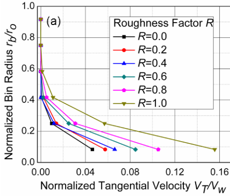
(Color online) Figure 6(a): Normalized velocity vs. radial location as a function of the roughness factor R .
