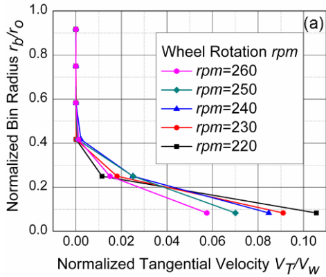
(Color online) Figure 7(a): Radial location vs. normalized tangential velocity as a function of wheel rotation (rpm).
