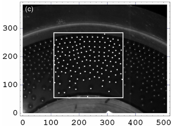
(Color online) Figure 4(c): The DPTV code computes the particle centroids in the area-of-interest indicated by the white box.
