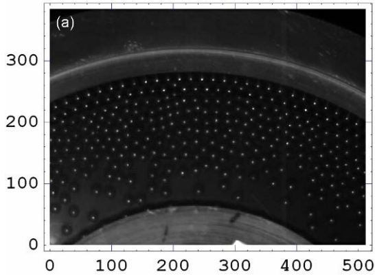
(Color online) Figure 4(a): An image extracted from high-speed video
