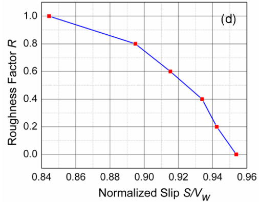
(Color online) Figure 6(d): Roughness factor vs. normalized slip.
