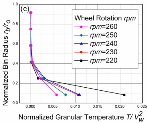
(Color online) Figure 7(c): Radial location vs. normalized granular temperature as a function of wheel rotation (rpm).
