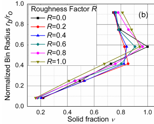
(Color online) Figure 6(b): Solid Fraction vs. radial location as a function of the roughness R .
