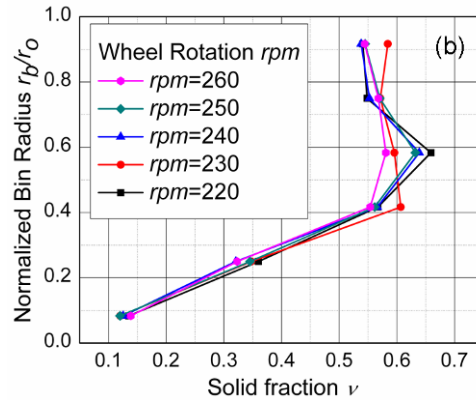
(Color online) Figure 7(b): Radial location vs. solid fraction as a function of wheel rotation (rpm).
