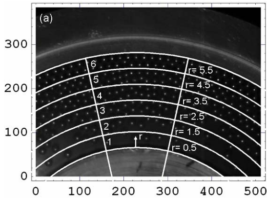
(Color online) Figure 5(a): The granular shear cell gap was divided into six radial bins, where bin-1 and bin-6 are adjacent to the inner (moving) and outer (stationary) surfaces, respectively.
