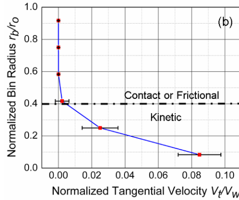
(Color online) Figure 5(b): Normalized radial position vs. the normalized tangential velocity. The dotted horizontal line delineates the transition from the granular frictional to kinetic regimes.
