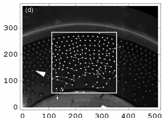
(Color online) Figure 4(d): The DPTV code also computes the particle velocity vectors that lead to granular flow parameters
